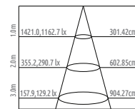
Lux Distance Curve
