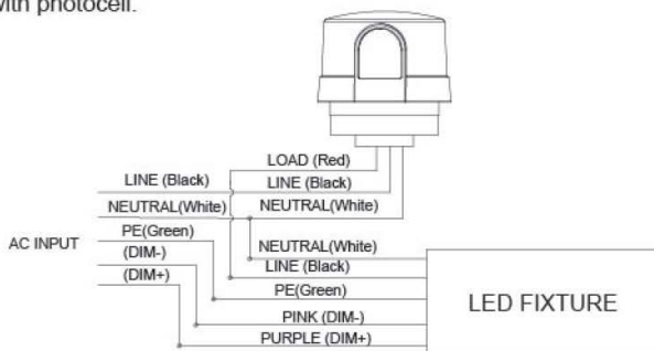
Wiring diagram with photocell.
