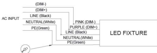
Wiring diagram without photocell and motion sensor.
