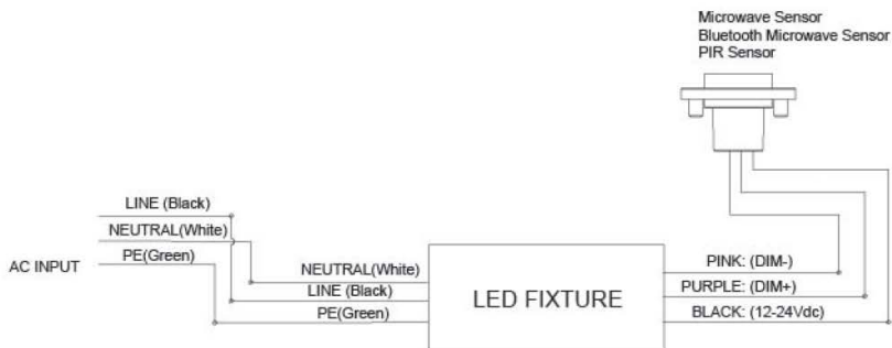
Wiring diagram with motion sensor.
