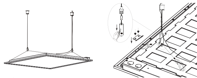
L2850-0002 Suspension cable kit for 2x2 L2850-0003 Suspension cable kit for 1x4 and 2x4 (Sold separately)
